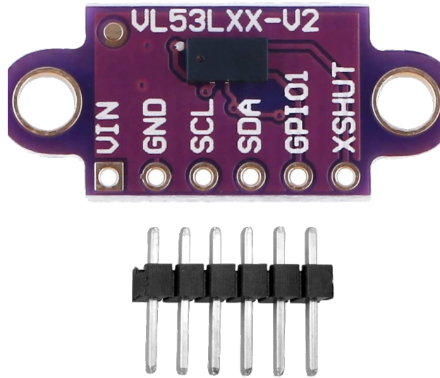
Figura 4 – Sensor VL53L0X
